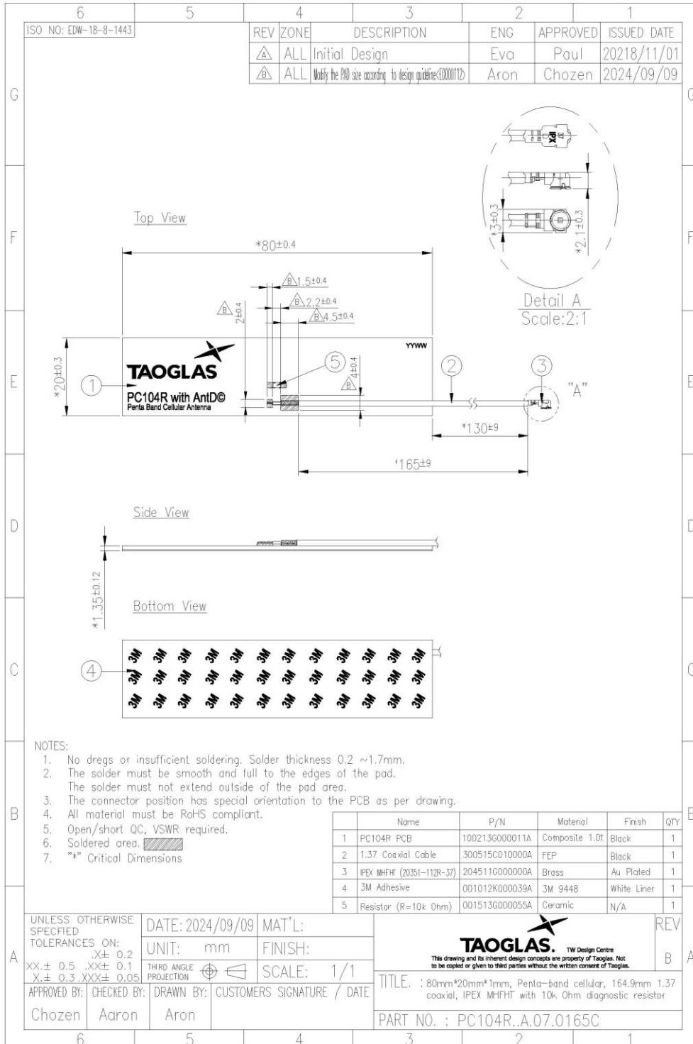
Figure 8. Mechanical Drawing for the PC104 Antenna
