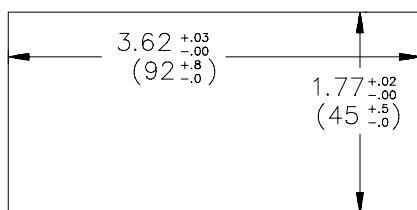
PANEL CUT-OUT
