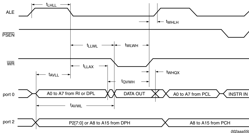
Fig 32. External data memory write cycle
