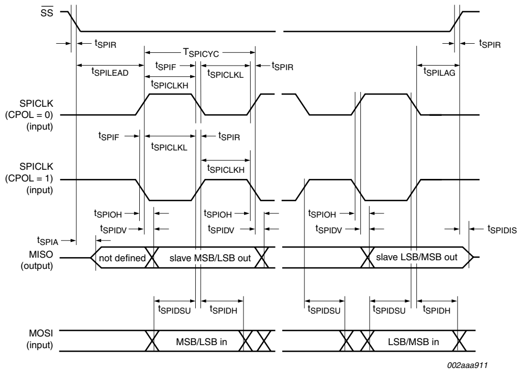
Fig 38. SPI slave timing (CPHA = 1)
