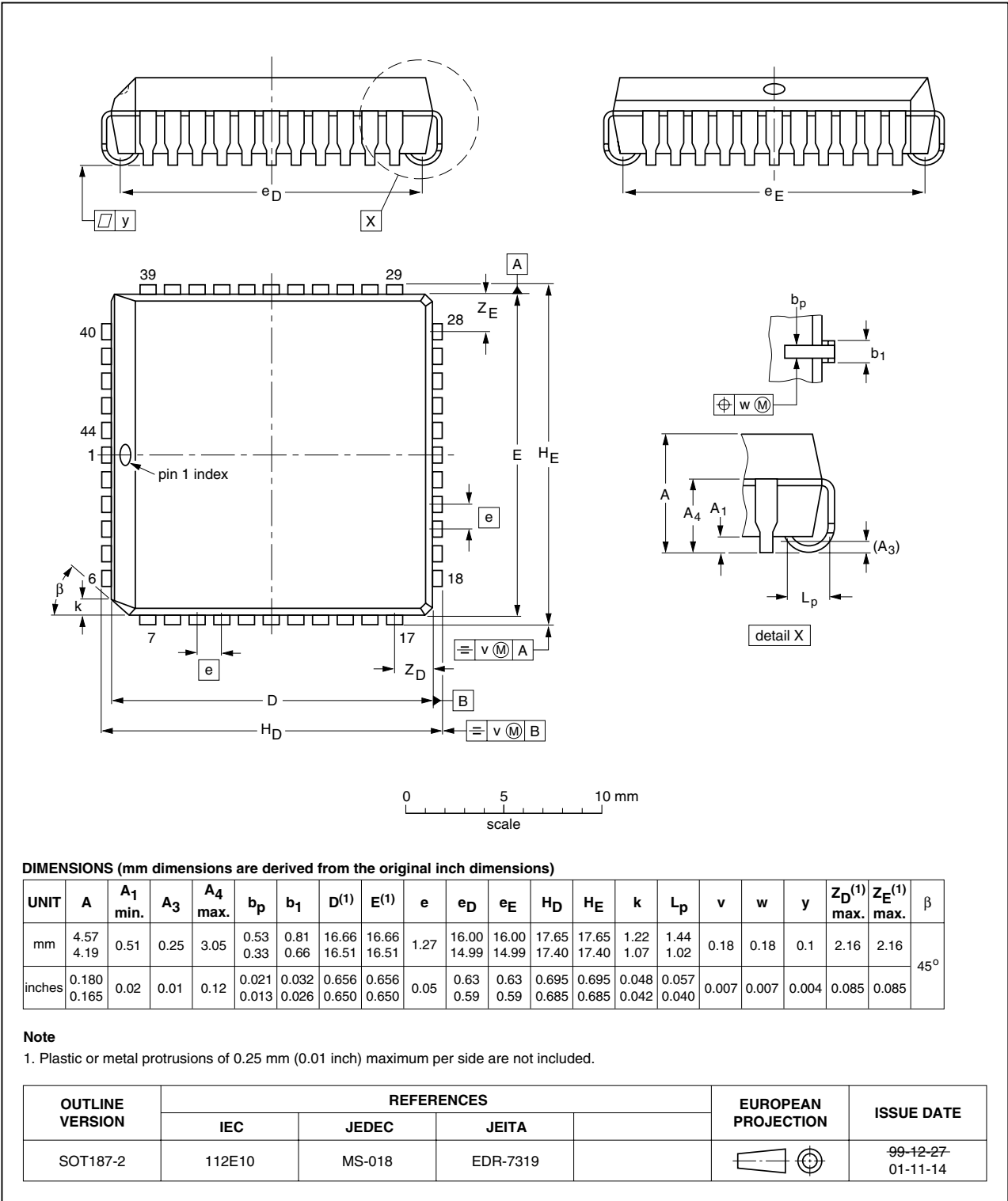
Fig 45. SOT187-2 (PLCC44) package outline
