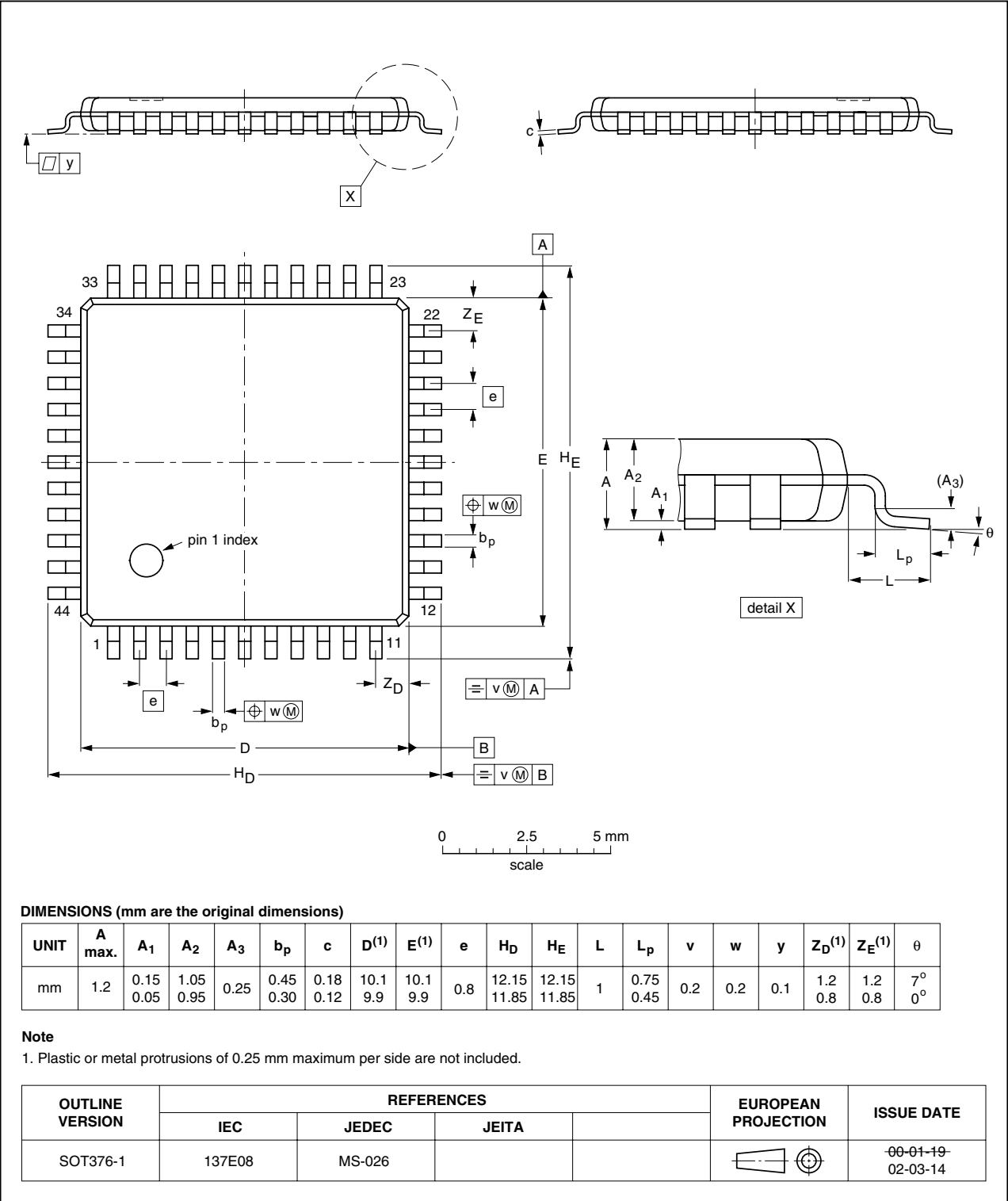
Fig 44. SOT376-1 (TQFP44) package outline
