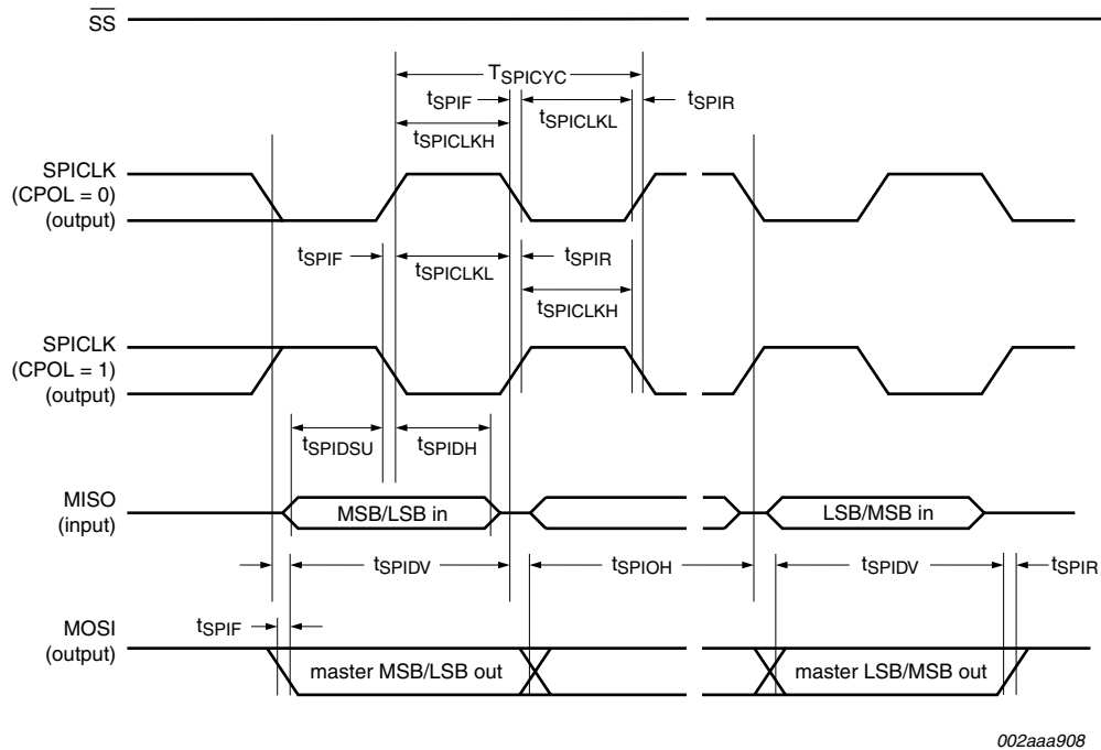
Fig 35. SPI master timing (CPHA = 0)
