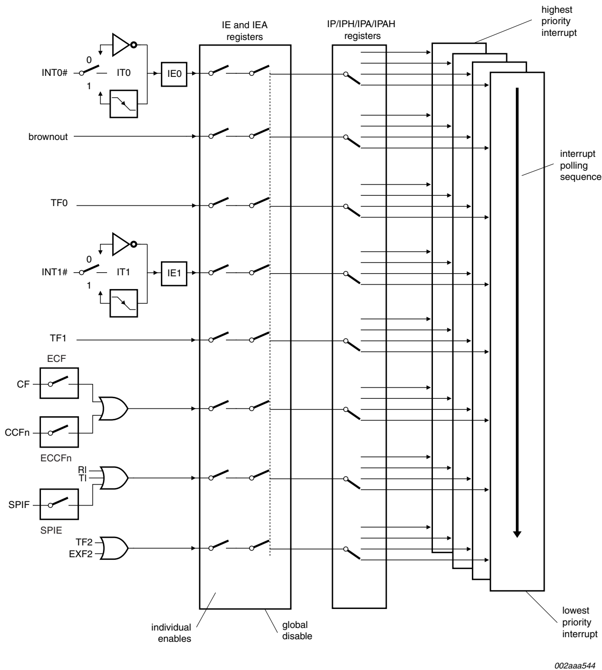
Fig 27. Interrupt structure
