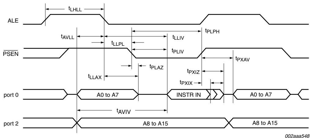
Fig 30. External program memory read cycle
