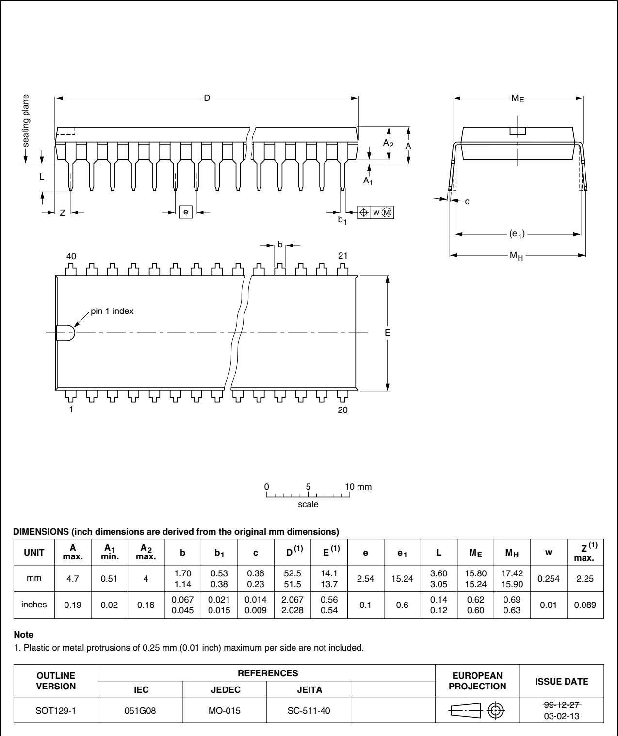
Fig 43. SOT129-1 (DIP40) package outline
