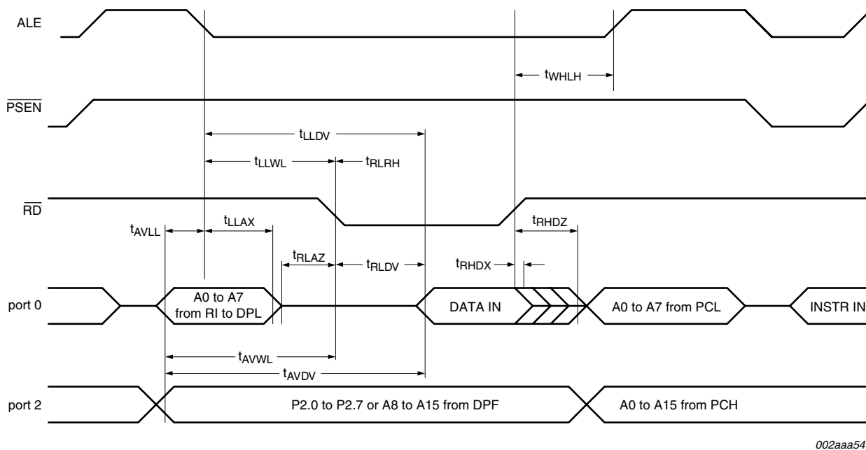
Fig 31. External data memory read cycle
