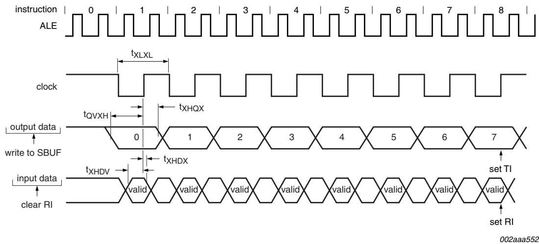
Fig 34. Shift register mode timing waveforms
