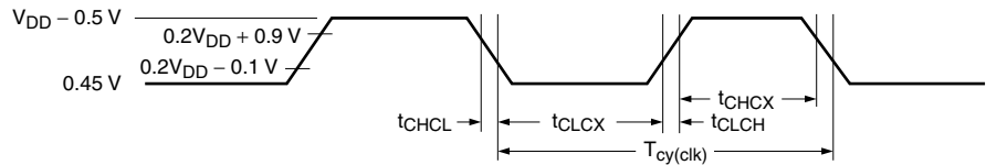
Fig 33. External clock drive waveform
