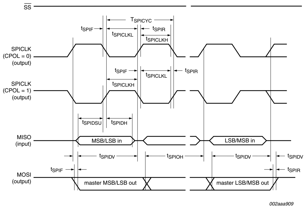
Fig 36. SPI master timing (CPHA = 1)
