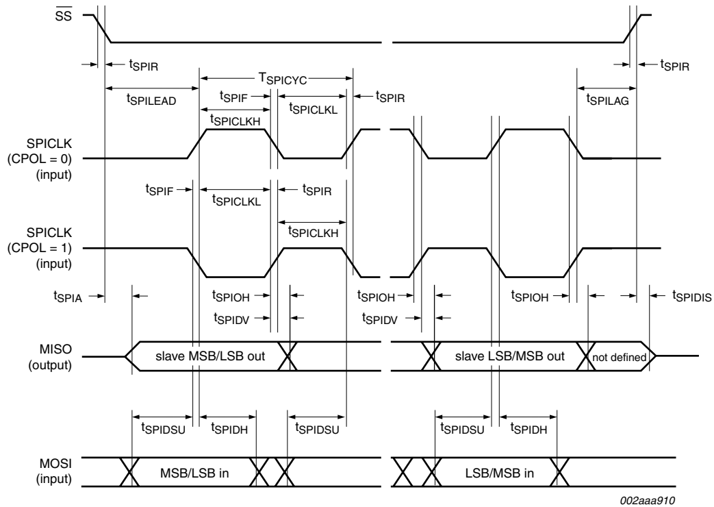
Fig 37. SPI slave timing (CPHA = 0)
