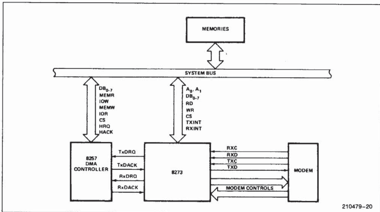
Figure 18. 8273 System Diagram
