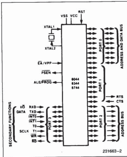
Figure 2. Logic Symbol
