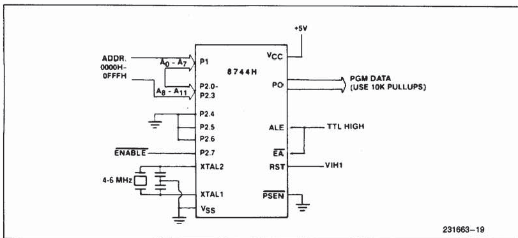
Figure 10. Program Verification Configuration
