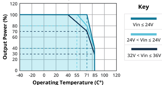
TEMPERATURE DERATING CURVE (12 Vdc output model)
