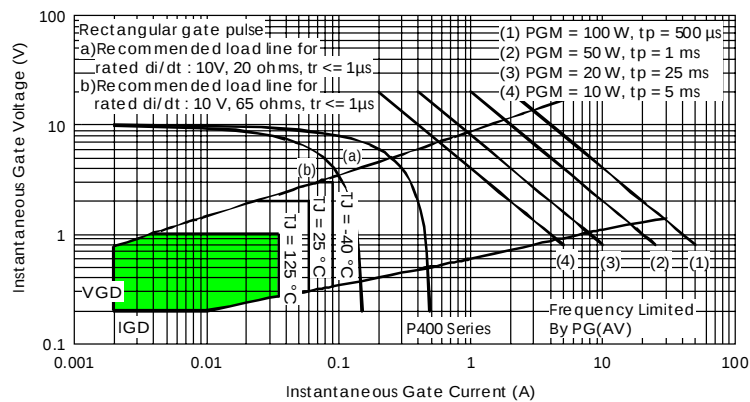
Fig. 9 - Gate Characteristics
