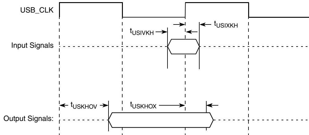
Figure 35. USB Signals
