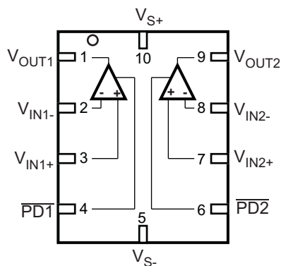
OPA2835 (TOP VIEW) WQFN-10 (RUN), UQFN-10 (RMC)
