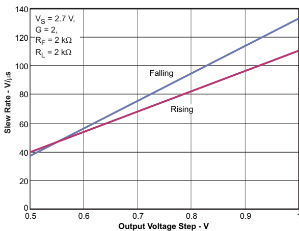
Figure 5. Slew Rate vs Output Voltage Step
