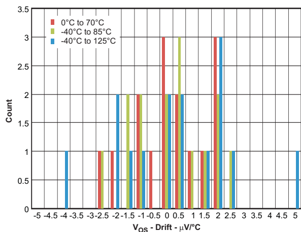
Figure 23. Input Offset Voltage Drift
