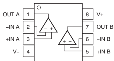
D and DGK (2) Packages: OPA2172 SOIC-8 and VSSOP-8 (Top View)
