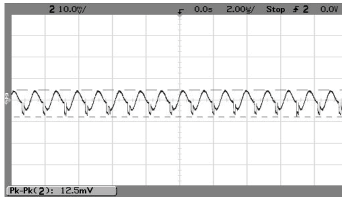
Output Ripple and Noise (Vin=14V, Vout=0.9V, Iout=1A, Cload=0, Ta=+25°C., ScopeBW=100MHz)
