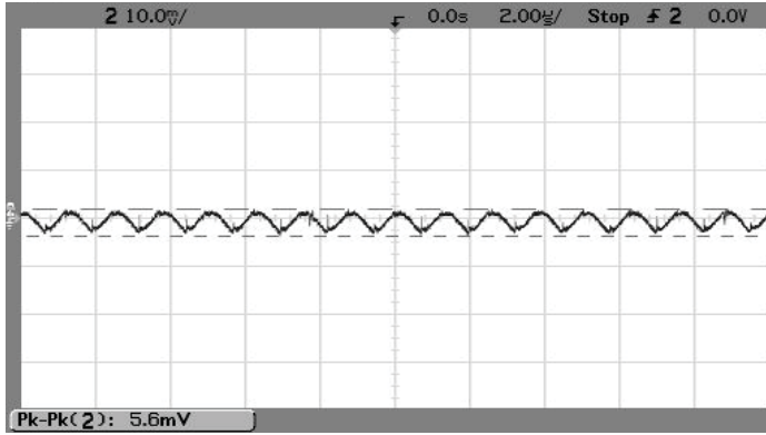
Output Ripple and Noise (Vin=2.6V, Vout=0.9V, Iout=1A, Cload=0, Ta=+25°C., ScopeBW=100MHz)
