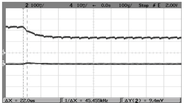
Step Load Transient Response (Vin=2.6V, Vout=0.9V, Cload=0, Iout=1A to 0.5A, Ta=+25°C.) Trace 2=Vout, 100 mV/div. Trace 4=Iout, 0.5A/div.
