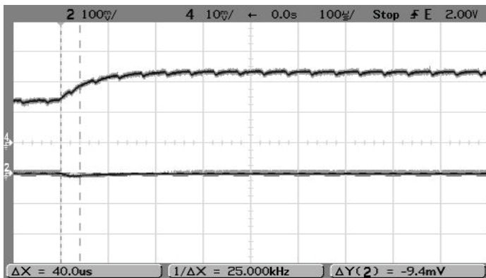
Step Load Transient Response (Vin=2.6V, Vout=0.9V, Cload=0, Iout=0.5A to 1A, Ta=+25°C.) Trace 2=Vout, 100 mV/div. Trace 4=Iout, 0.5A/div.
