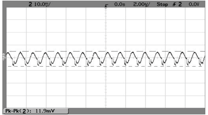
Output Ripple and Noise (Vin=12V, Vout=0.9V, Iout=1A, Cload=0, Ta=+25°C., ScopeBW=100MHz)
