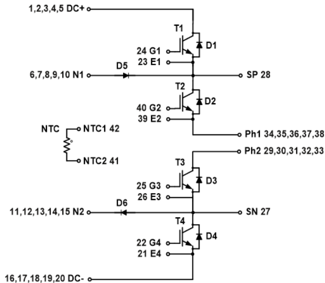
Figure 1. NXH400N100H4Q2F2PG/SG Schematic Diagram
