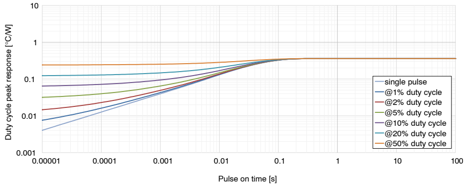
Figure 52. IGBT Transient Thermal Impedance
