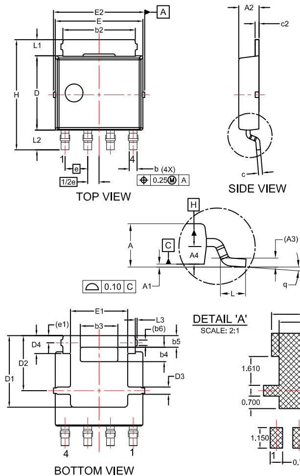
LFPAK4 5x6 CASE 760AB ISSUE C
