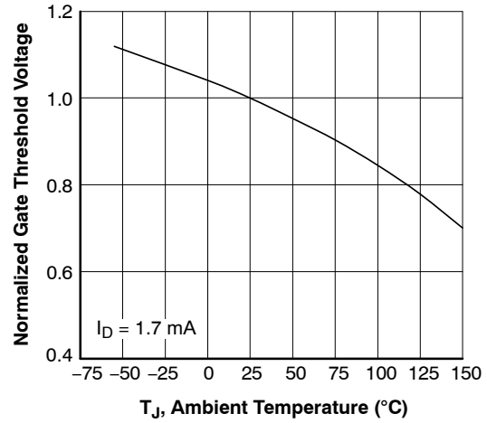
Figure 16. Normalized Gate Threshold Voltage vs. Temperature
