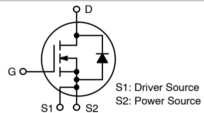
N-CHANNEL MOSFET
