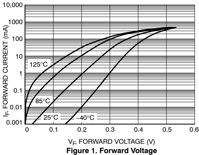
Figure 1. Forward Voltage
