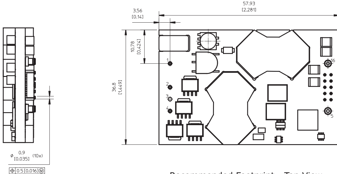
Recommended Footprint - Top View
