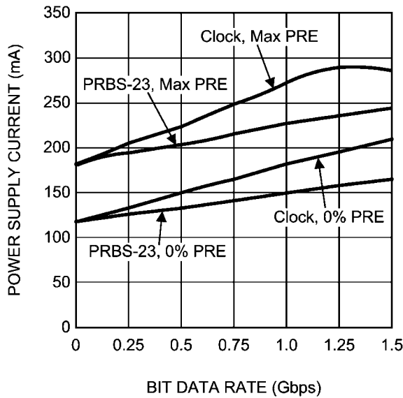
Power Supply Current vs. Bit Data Rate
