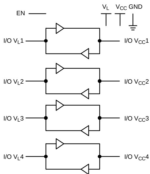
Figure 2. Logic Diagram
