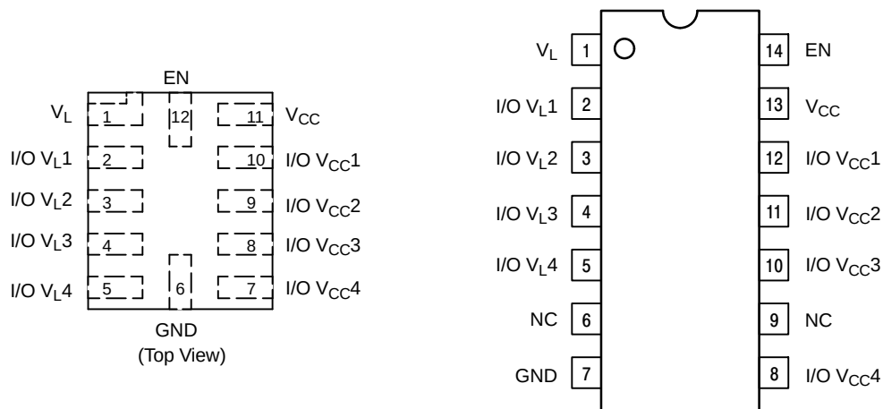
Figure 1. Pin Assignments
