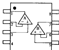
NJM4562D NJM4562M
