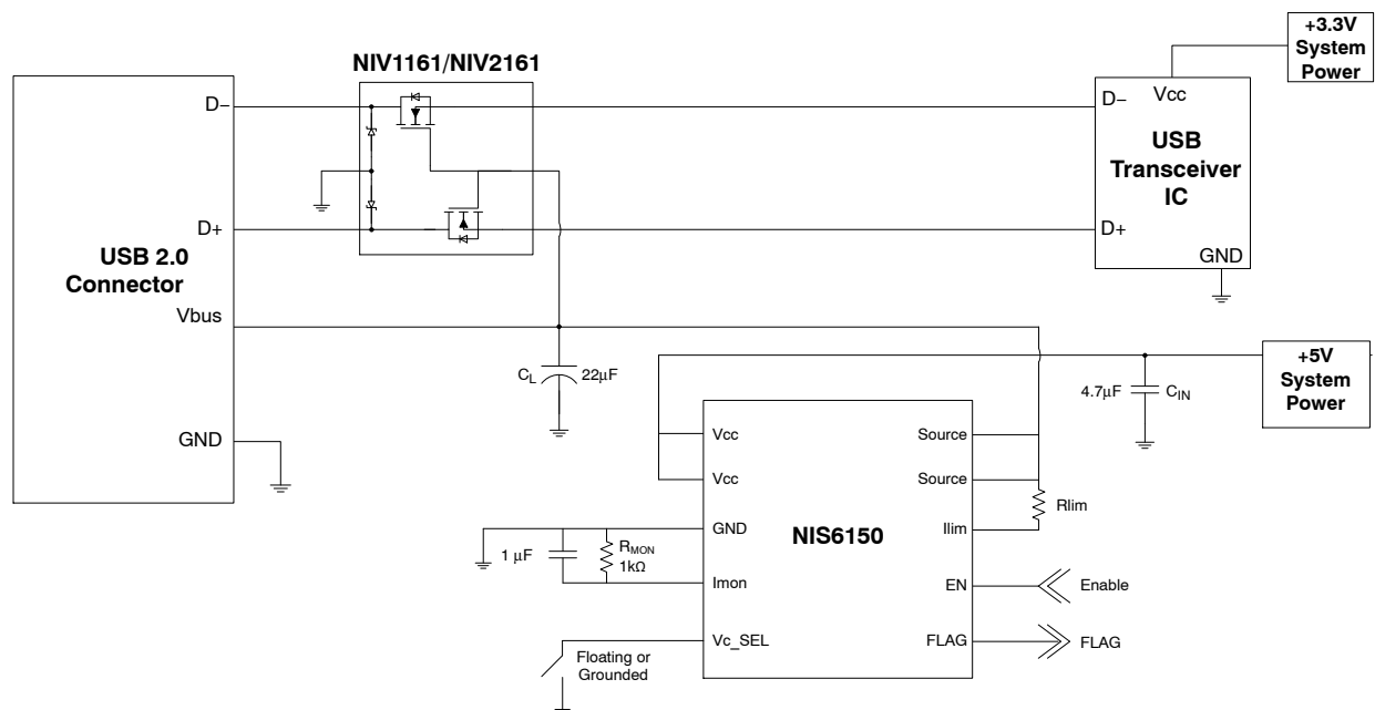
Figure 1. Typical USB 2.0 Application Circuit
