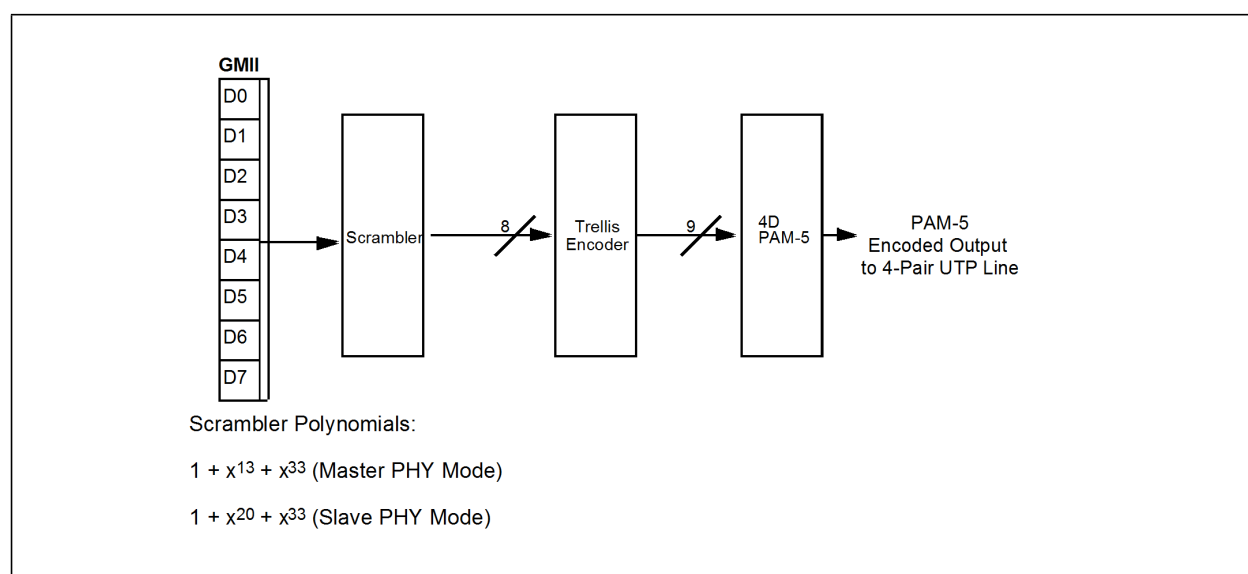
Figure 3-11 1000BASE-T Transmit Flow And Line Coding Scheme
