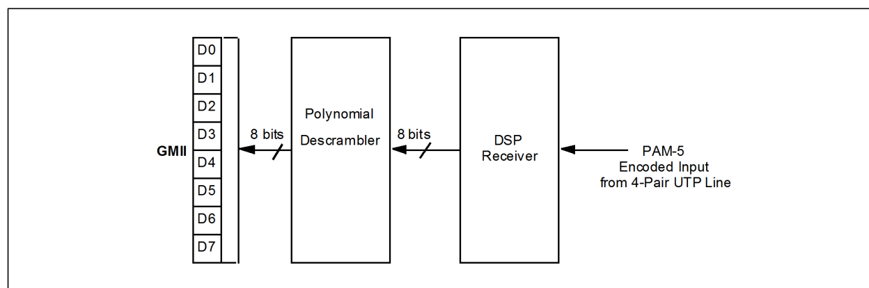
Figure 3-12 Transmit/Receive Flow
