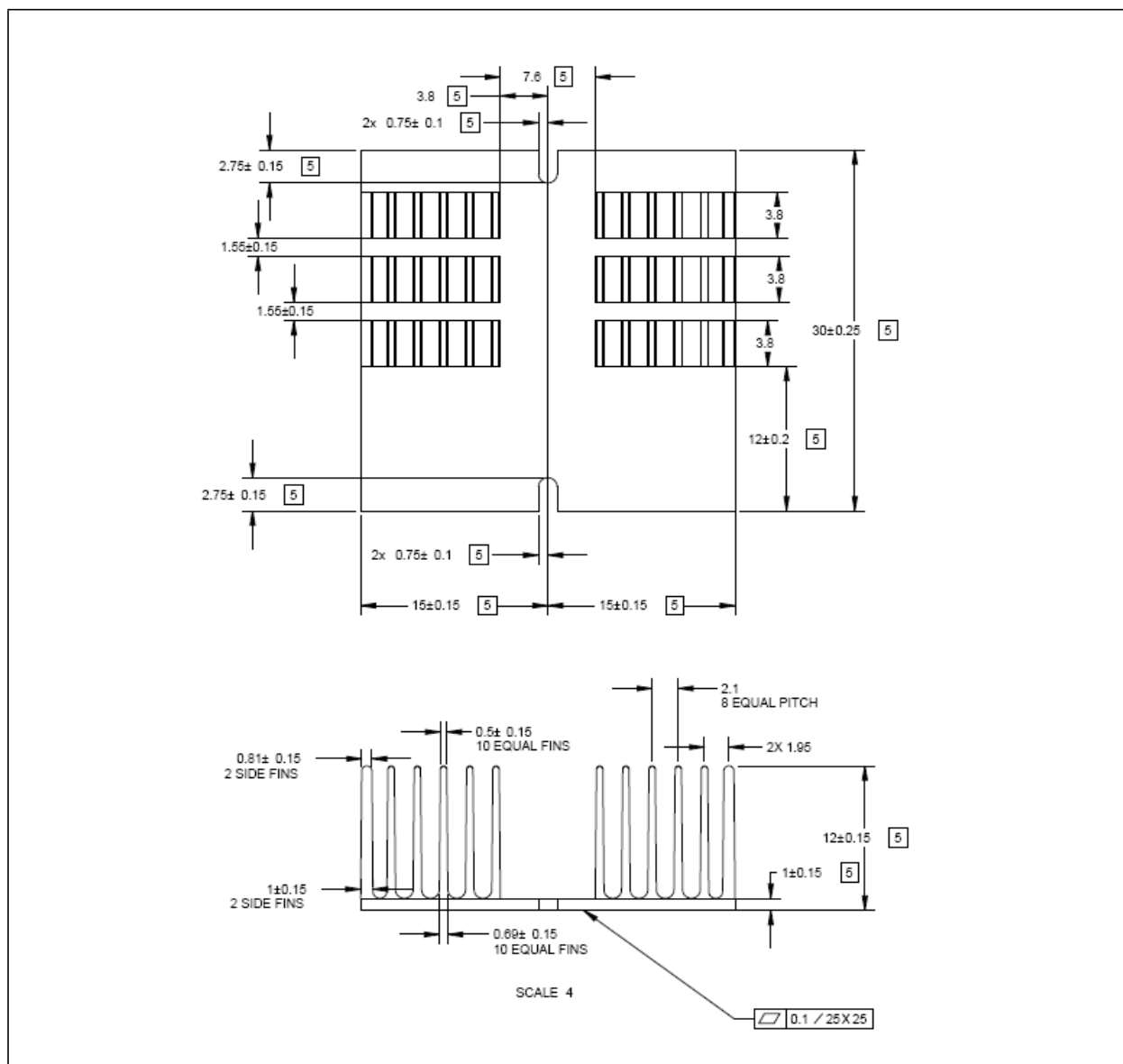
Figure 13-2 Rose City 12 mm Height Passive Heat Sink
