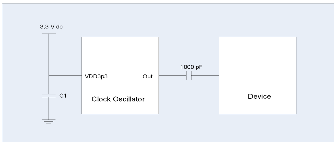
Figure 12-6 Oscillator Solution
