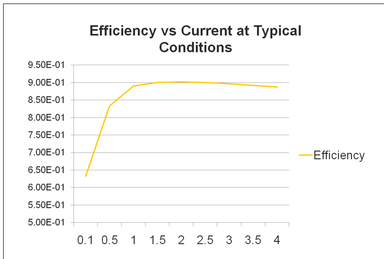
Figure 11-15 SVR Efficiency
