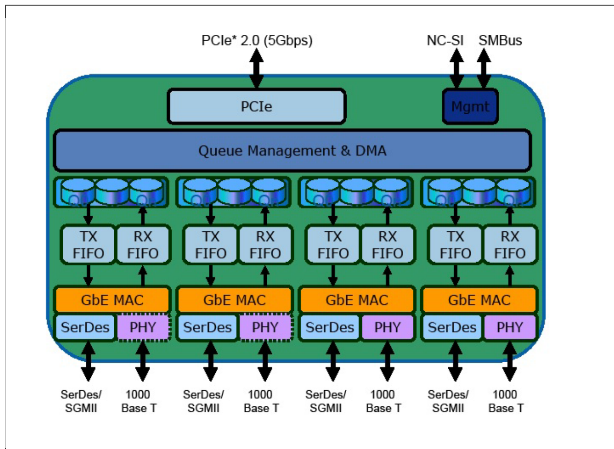
Figure 1-1 Intel® Ethernet Controller I350
