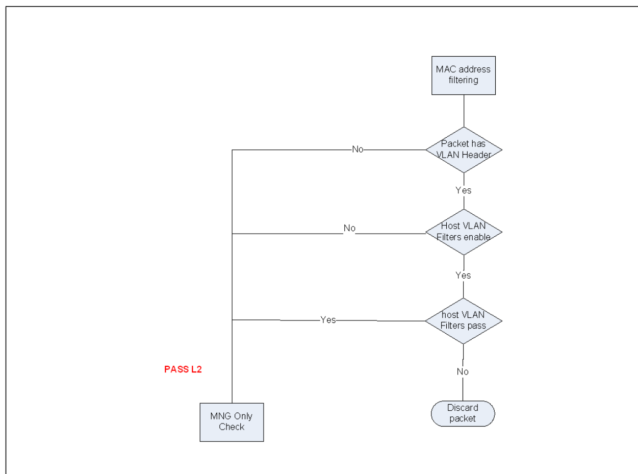
Figure 7-4 VLAN Filtering
