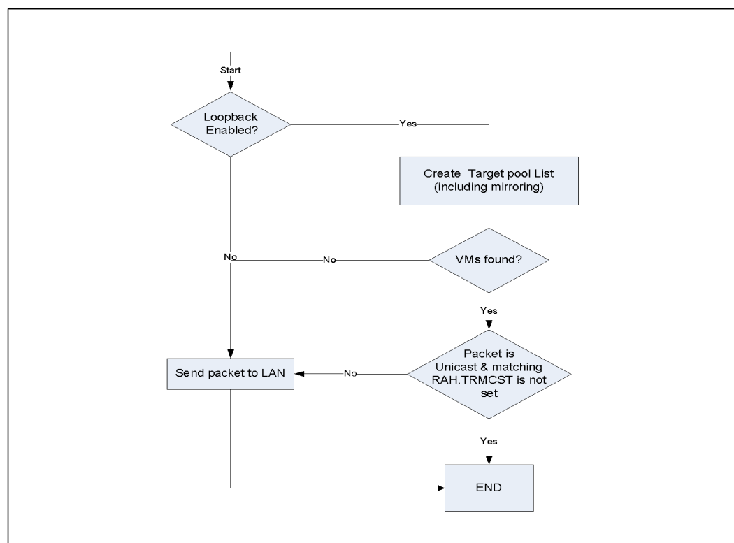
Figure 7-25 Tx Filtering
