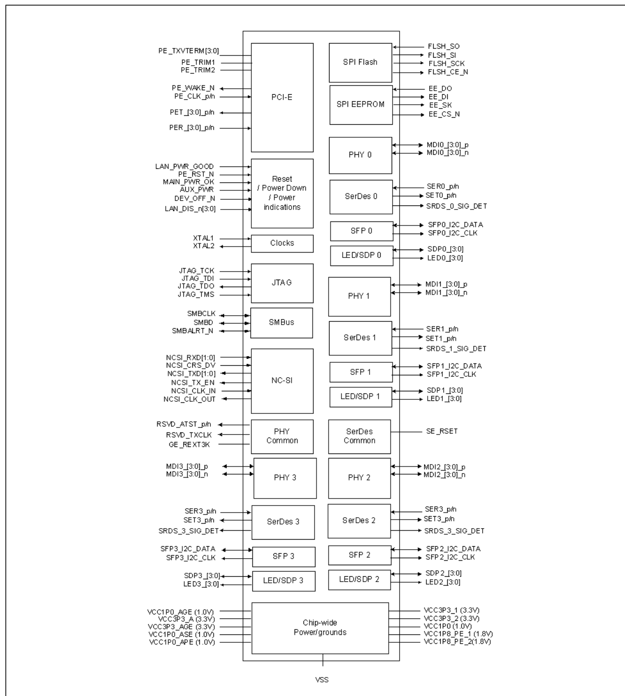
Figure 2-1 I350 Interface Diagram
