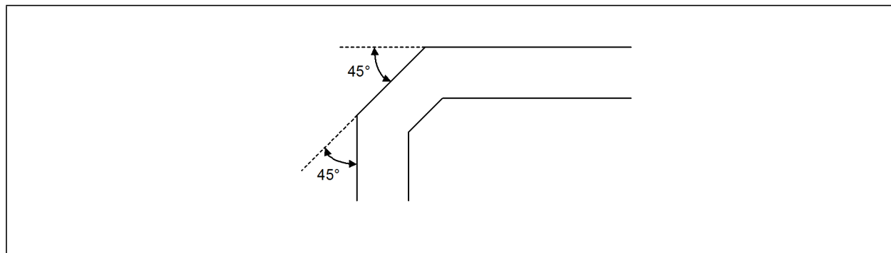
Figure 12-3 Trace Routing
