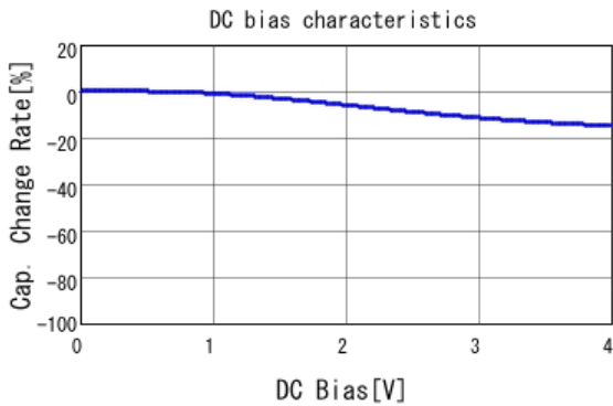
■ NFM18HC106D0G3 C-DC bias capchange, 25.0degC, AC0.5Vr
