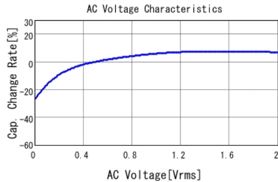
■ NFM18HC106D0G3 C-AC Voltage capchange, DC0V, 25.0degC
