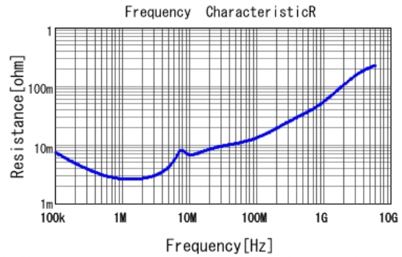
■ NFM18HC106D0G3 R DC0V, 25degC, Non-feedthrough
