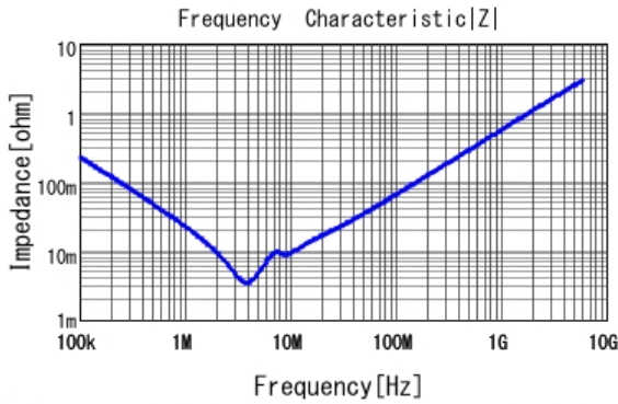
■ NFM18HC106D0G3 |Z| DC0V, 25degC, Non-feedthrough
