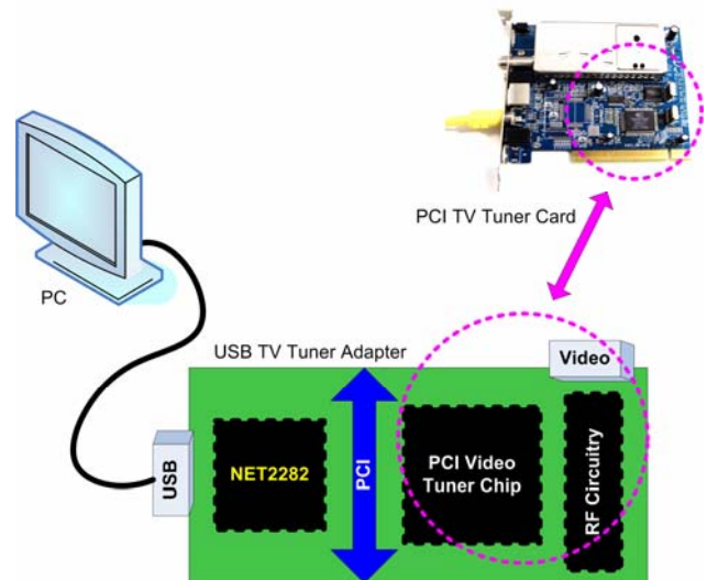
Figure 2: Converting a PCI TV Tuner Board to USB
