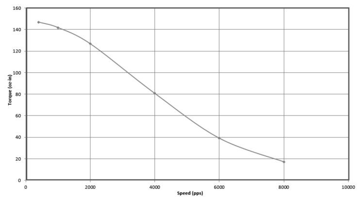
CUI P/N NEMA23-31-01PD-AMT112S Lin Engineering P/N WO-5718L-01P (1.8 Step Motor) 24 Vdc, 2.8 Amp/Phase, IB463, 1/2 Stepping
