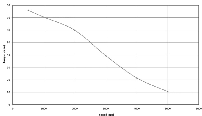
CUI P/N NEMA23-17-01SD-AMT112S Lin Engineering P/N WO-5718X-01S (1.8 Step Motor) 24 Vdc, 1.4 Amp/Phase, Bipolar, 1/2 Stepping
