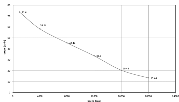
CUI P/N NEMA23-17-01PD-AMT112S Lin Engineering P/N WO-5718X-01P (1.8 Step Motor) 24 Vdc, 2.8 Amp/Phase, IB463, 1/2 Stepping
