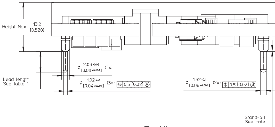
Top View Pin Positions According To Recommended Footprint
