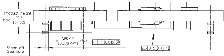
Top View Pin Positions According To Recommended Footprint
