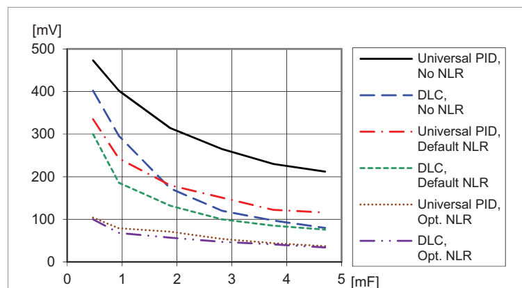
Load Transient vs. External Capacitance, V_O = 1.0 V
