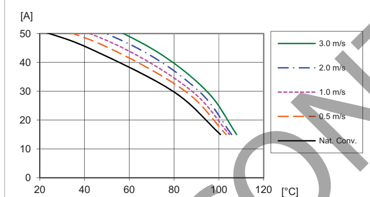
Output Current Derating, V_O = 1.8\text{ V}
