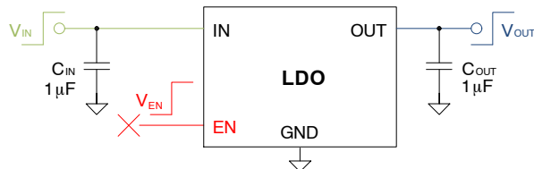
Figure 62. Circuit – Floating EN Pin
