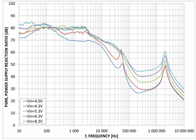
Figure 43. PSRR – NCV8730–3.3 V, C_{OUT} = 1\text{ }\mu\text{F} , I_{OUT} = 100\text{ mA}
