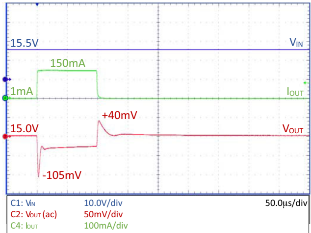
Figure 29. Load Transient – NCV8730–15.0 V, C_{OUT} = 10\text{ }\mu\text{F}
