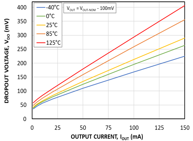
Figure 15. NCV8730ASN330 – Dropout Voltage
