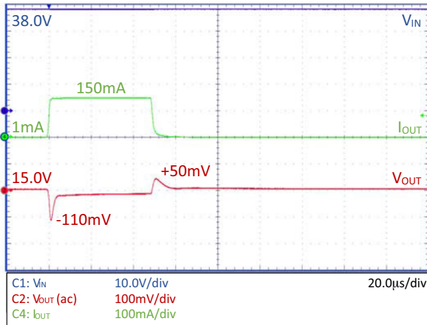
Figure 28. Load Transient – NCV8730–15.0 V, C_{OUT} = 1\text{ }\mu\text{F}
