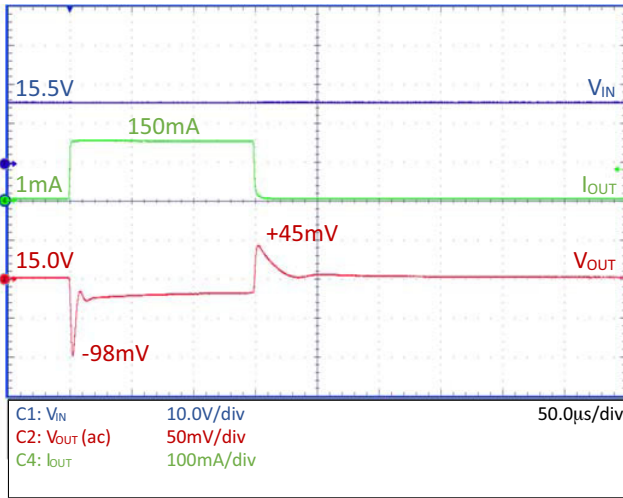
Figure 30. Load Transient – NCV8730–15.0 V, C_{OUT} = 22\text{ }\mu\text{F}
