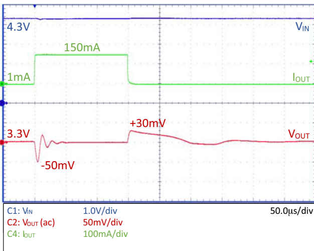
Figure 22. Load Transient – NCV8730–3.3 V, C_{OUT} = 22\text{ }\mu\text{F}
