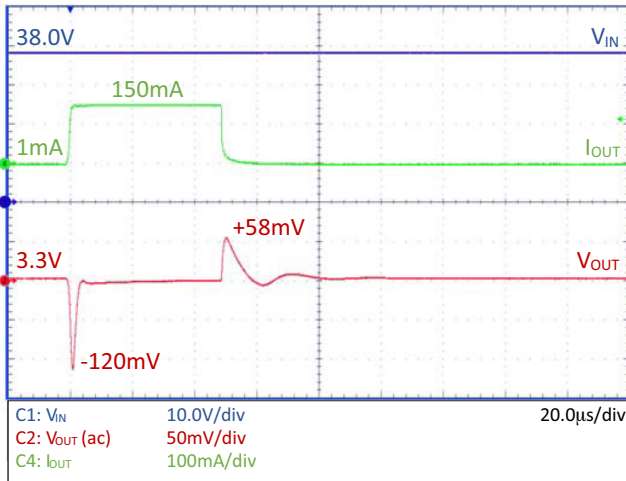
Figure 20. Load Transient – NCV8730–3.3 V, C_{OUT} = 1\text{ }\mu\text{F}
