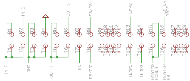
Figure 88. Edge Connector Pinout (All Demo Boards)
