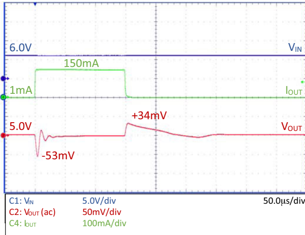
Figure 26. Load Transient – NCV8730–5.0 V, C_{OUT} = 22\text{ }\mu\text{F}
