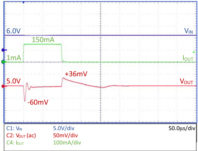
Figure 25. Load Transient – NCV8730–5.0 V, C_{OUT} = 10\text{ }\mu\text{F}
