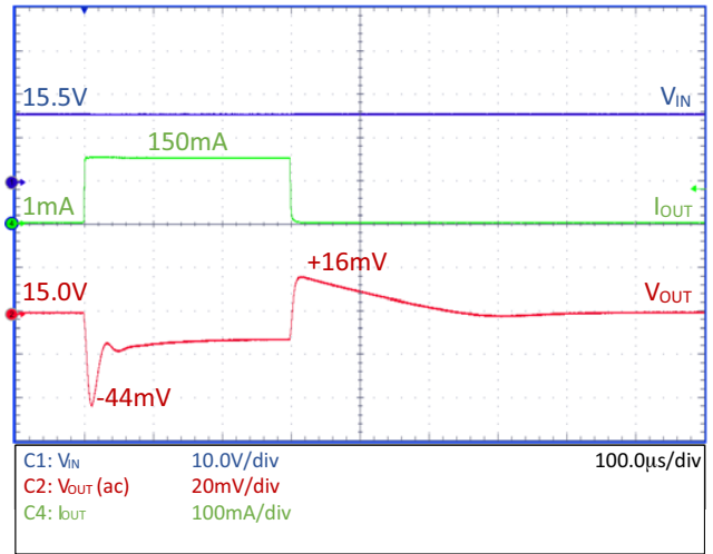
Figure 31. Load Transient – NCV8730–15.0 V, C_{OUT} = 50\text{ }\mu\text{F}
