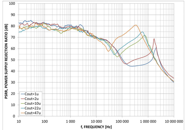
Figure 45. PSRR – NCV8730–3.3 V, V_{IN} = 8.3\text{ V} , I_{OUT} = 100\text{ mA}
