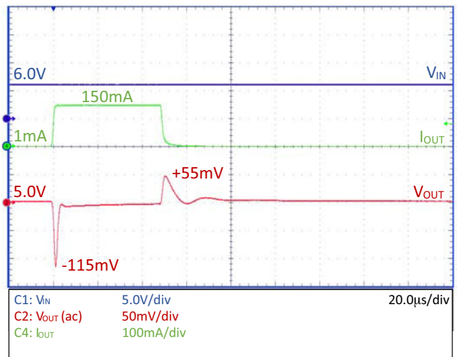
Figure 23. Load Transient – NCV8730–5.0 V, C_{OUT} = 1\text{ }\mu\text{F}
