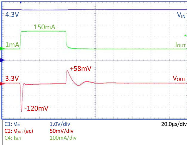
Figure 18. Load Transient – NCV8730–3.3 V, C_{OUT} = 1\text{ }\mu\text{F}
