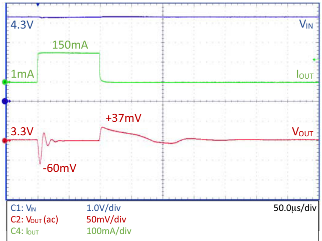
Figure 21. Load Transient – NCV8730–3.3 V, C_{OUT} = 10\text{ }\mu\text{F}
