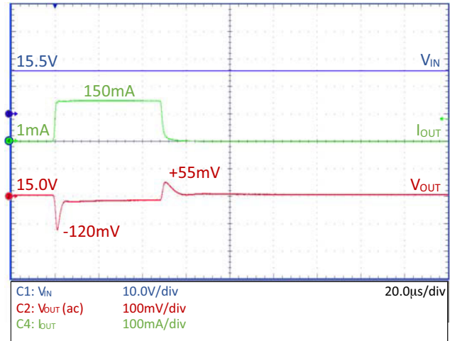
Figure 27. Load Transient – NCV8730–15.0 V, C_{OUT} = 1\text{ }\mu\text{F}
