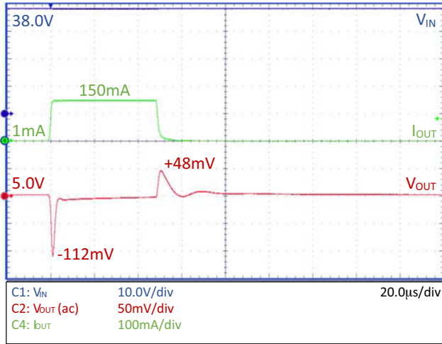
Figure 24. Load Transient – NCV8730–5.0 V, C_{OUT} = 1\text{ }\mu\text{F}
