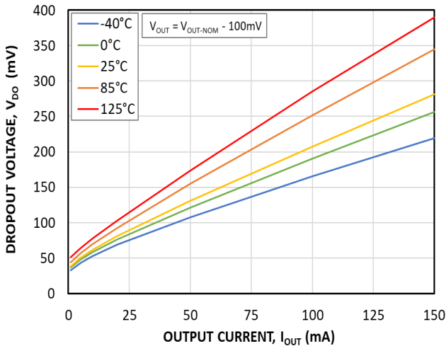
Figure 16. NCV8730BMT500 – Dropout Voltage
