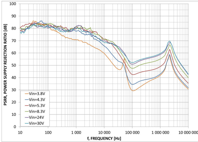
Figure 42. PSRR – NCV8730–3.3 V, C_{OUT} = 1\text{ }\mu\text{F} , I_{OUT} = 10\text{ mA}
