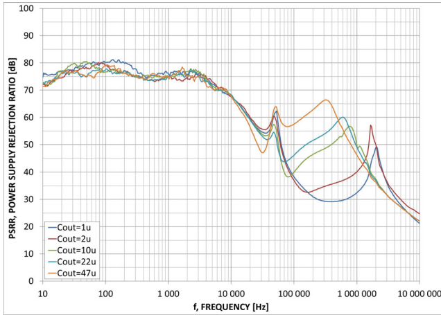
Figure 44. PSRR – NCV8730–3.3 V, V_{IN} = 4.3\text{ V} , I_{OUT} = 100\text{ mA}
