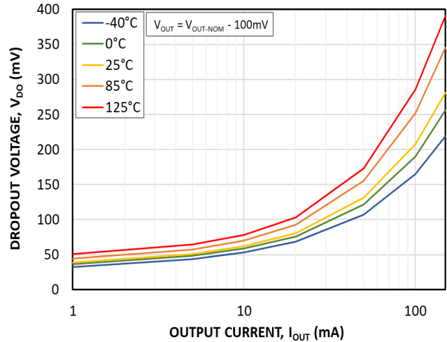
Figure 17. NCV8730BMT500 – Dropout Voltage
