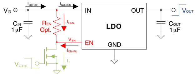
Figure 70. Circuit – EN Pin Controlled by Transistor
