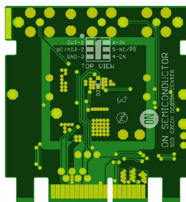
Figure 96. WDFN-6 2x2 Demo Board (2 layer, rev. 1) – PCB Bottom Layer
