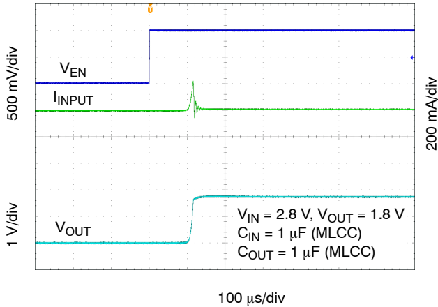
Figure 28. Enable Turn-on Response – C_{OUT} = 1\text{ μF} , I_{OUT} = 10\text{ mA}
