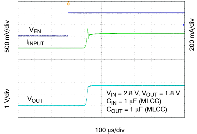
Figure 29. Enable Turn-on Response – C_{OUT} = 1\text{ μF} , I_{OUT} = 250\text{ mA}
