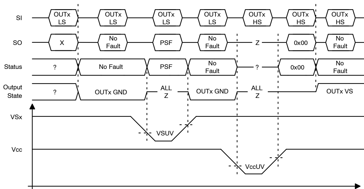
Figure 21. Undervoltage Timing
