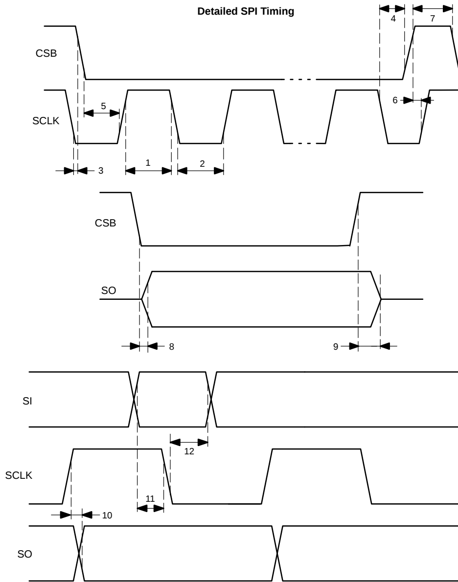
Figure 8. SPI Timing Waveforms
