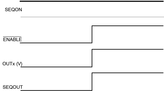
Figure 28. Sequence Interrupt from \overline{\text{EN}}
