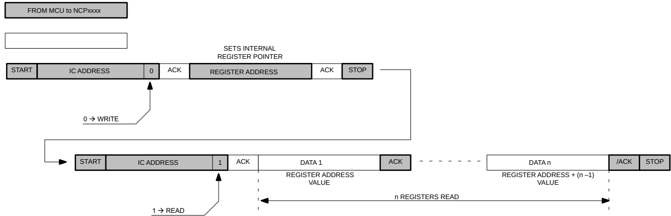
Figure 51. Read Sequence
