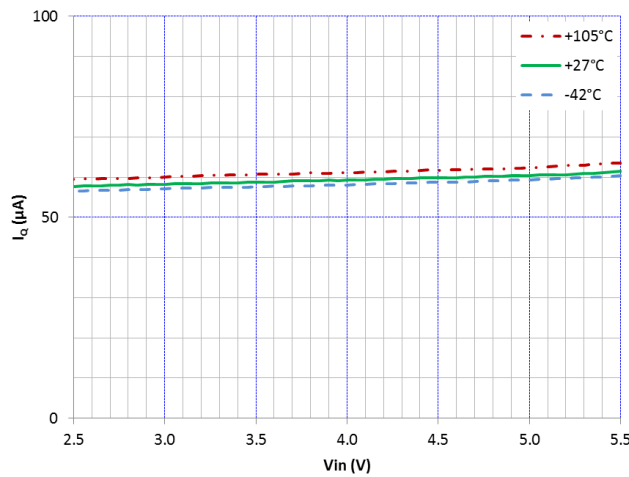
Figure 25. I_{Q\_PFM} vs V_{IN} and Temperature V_{OUT} = 1.25\text{ V}
