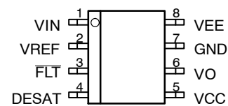
NCV5705B
