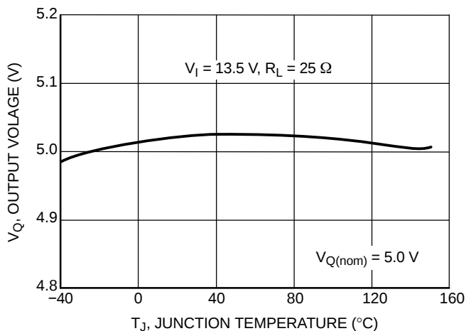
Figure 6. Output Voltage V_Q vs. Temperature T_J
