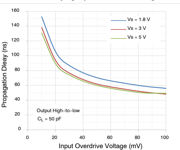
Figure 6. Output High-to-Low Propagation Delay vs. Input Overdrive Voltage
