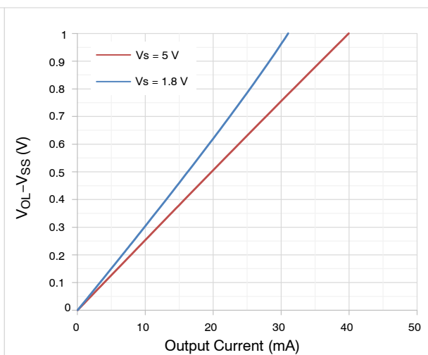
Figure 14. Output Voltage Low vs. Output Current
