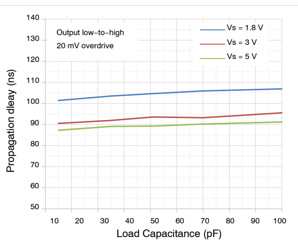
Figure 8. Output Low-to-High Propagation Delay vs. Load Capacitance
