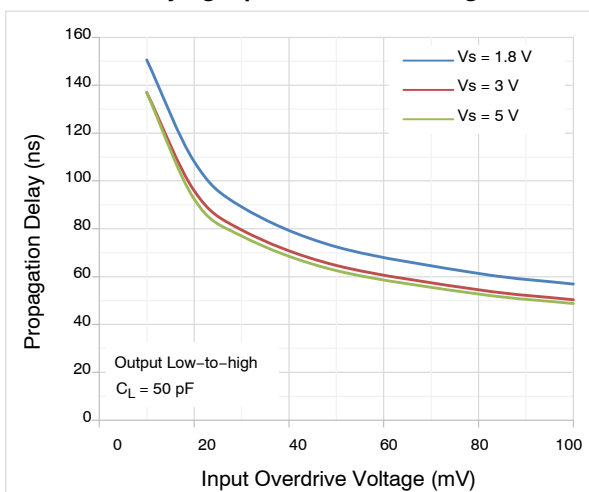
Figure 5. Output Low-to-High Propagation Delay vs. Input Overdrive Voltage
