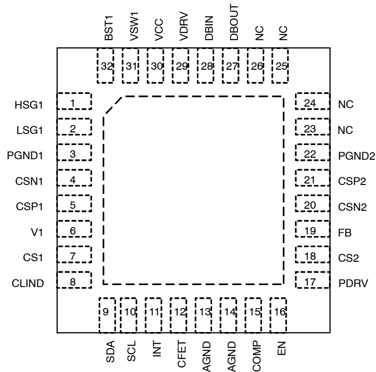
Figure 3. Pinout
