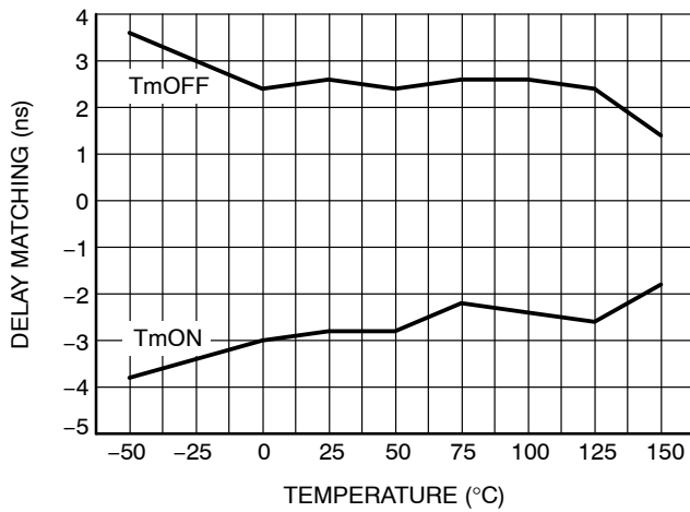
Figure 6. Delay Matching vs. Temperature
