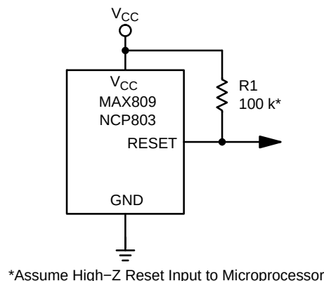
Figure 14. RESET Signal Integrity
