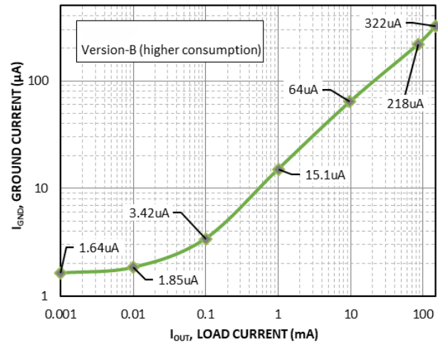
Figure 7. Ground Current vs. Load Current (NCP730-5.0V, Version-B)
