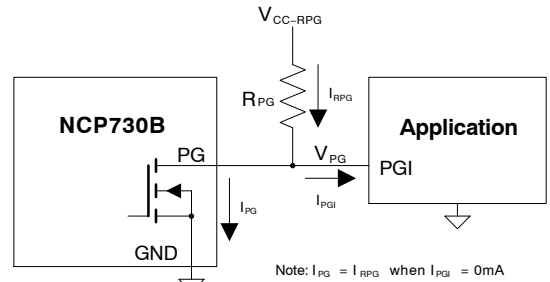
Figure 82. Circuit Example for R_{PG} Value Selection
