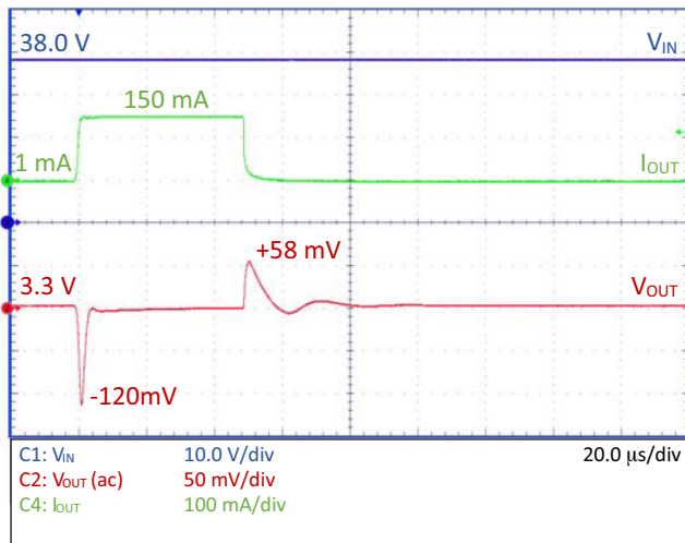
Figure 20. Load Transient – NCP730–3.3 V, C_{OUT} = 1\text{ }\mu\text{F}
