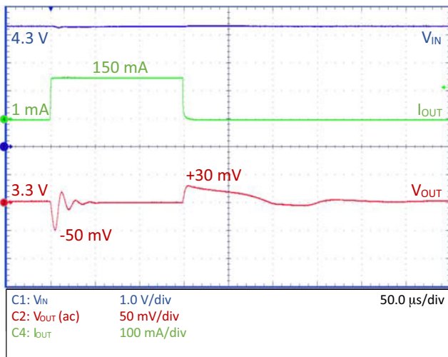
Figure 22. Load Transient – NCP730–3.3 V, C_{OUT} = 22\text{ }\mu\text{F}
