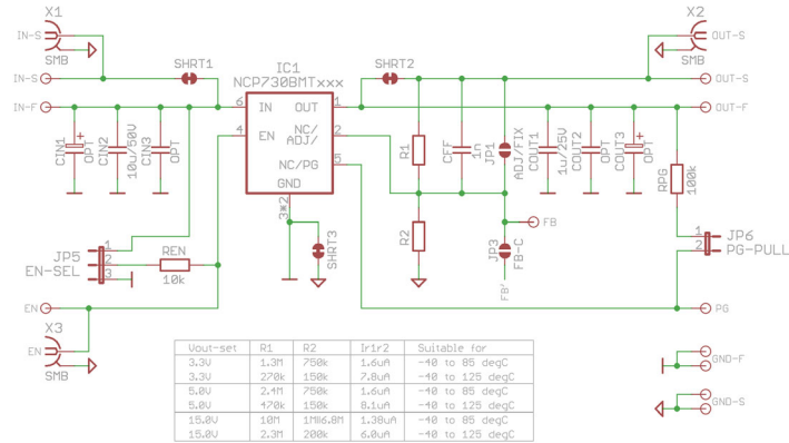
Figure 94. WDFN-6 2x2 Demo Board (2 layer, rev. 1) – Schematics (Main Part)
