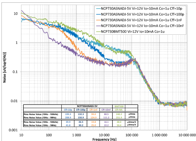
Figure 52. Noise – ADJ-set-5.0 V with Different C_{FF} and FIX – 5.0 V
