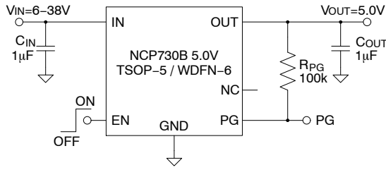
Figure 3. Fixed Output Voltage Application with PG
