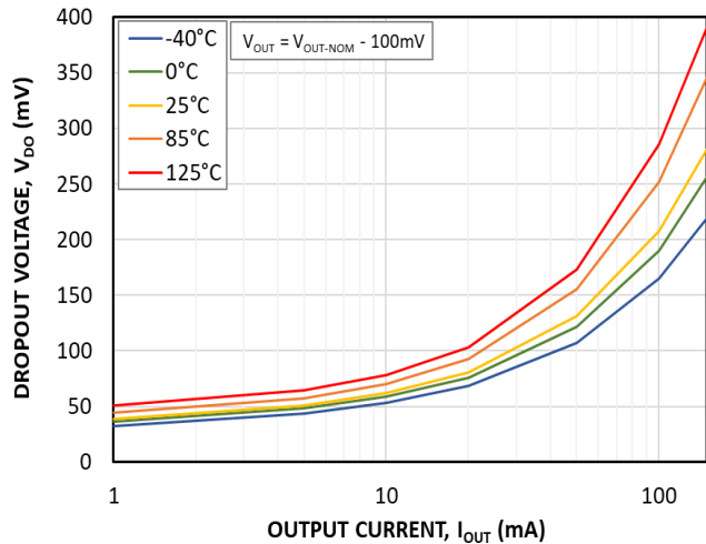
Figure 17. NCP730BMT500 - Dropout Voltage Detail
