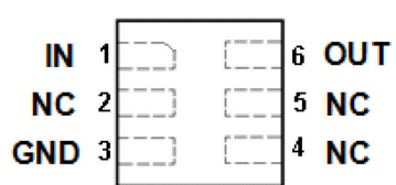
Figure 3. Pin Description
