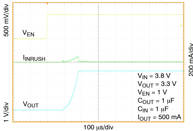
Figure 42. Enable Turn-on Response, C_{OUT} = 1 \mu\text{F} , I_{OUT} = 10 \text{ mA}
