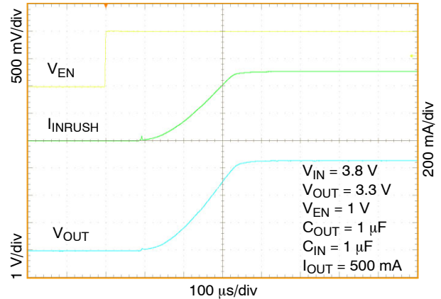
Figure 43. Enable Turn-on Response, C_{OUT} = 1 \mu\text{F} , I_{OUT} = 500 \text{ mA}
