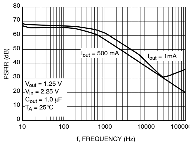
Figure 16. PSRR vs. Frequency ( V_{out} = 1.25 V)
