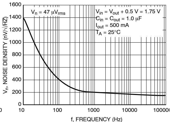
Figure 18. Noise Density vs. Frequency ( V_{out} = 1.25 V)
