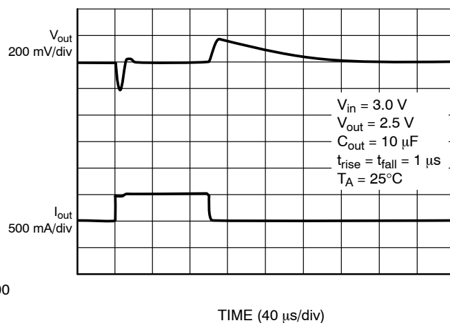
Figure 20. Load Transient ( V_{out} = 2.5 V)
