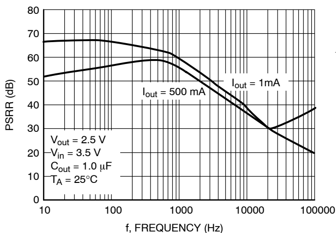
Figure 17. PSRR vs. Frequency ( V_{out} = 2.5 V)
