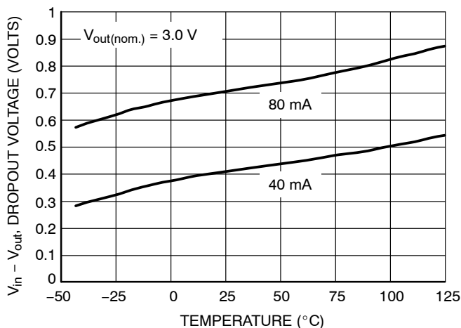
Figure 2. Dropout Voltage versus Temperature
