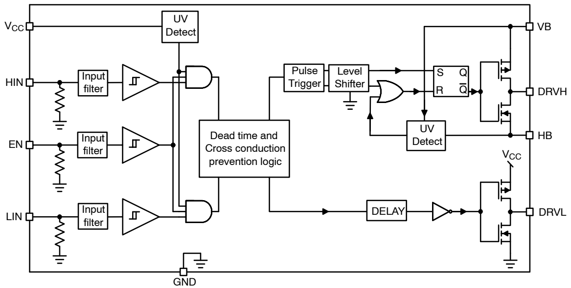
Figure 3. NCP51513B Version
