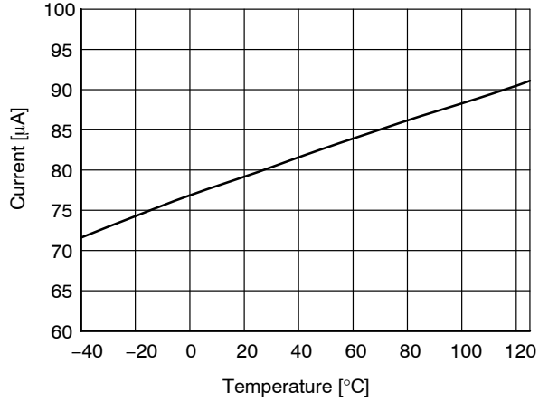
Figure 18. I_{B1\ EN\ H} vs. Temperature
