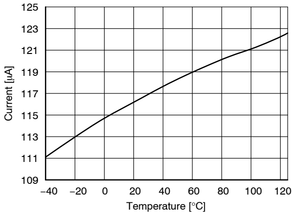
Figure 14. I_{CC1 \text{ EN H}} vs. Temperature
