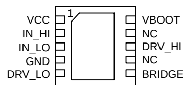
DFN-10
