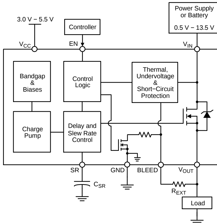
Figure 33. NCP4521 Typical Application Diagram – Load Switch
